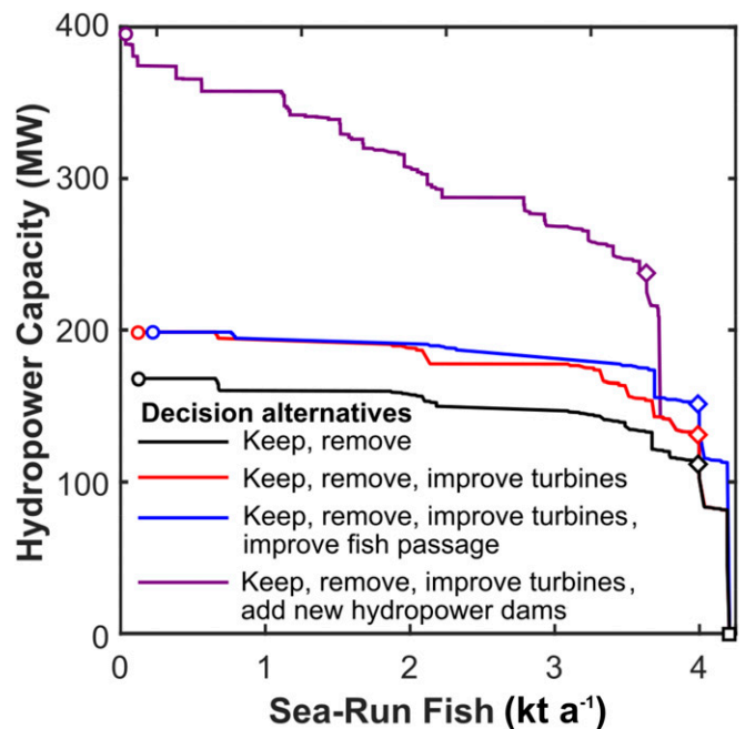
Fig. 3. PPFs for Penobscot depicting improvements in trade-off patterns associated with multiple decision alternatives. Hydropower capacity expansion based on turbine improvement estimates (33), fish passage expansion assumes survival rates improve by 50%. We include 54 candidate sites for the “add new hydropower dams” decision alternative (34).
